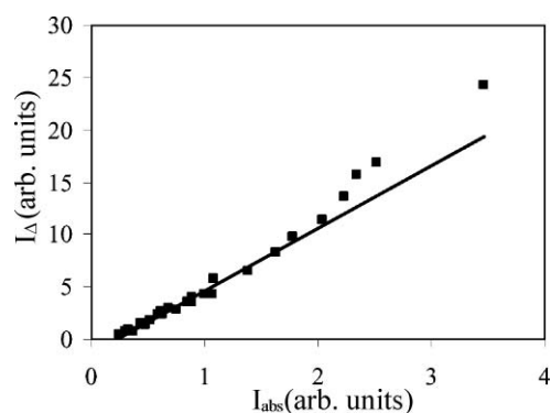
Fig. 6 Phosphorescence intensity versus the integrated light absorption for BOPP-Fb in acetone. I_{\text{abs}} values were calculated using eqn (2). The phosphorescence intensity was monitored at 1278 nm.
