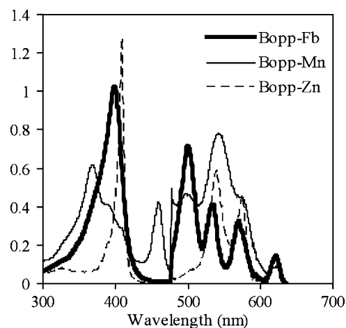
Fig. 2 Absorption spectra of BOPP in methanol before and after the inclusion of \text{Mn}^{2+} and \text{Zn}^{2+} into the macrocyclic core of the porphyrin molecule. The Q-band region of the spectrum has been enhanced by a factor of 10 for clarity.
